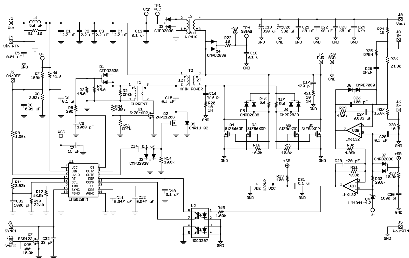
Figure 34. Application Circuit: Input 36-78V, Output 3.3V, 30A
